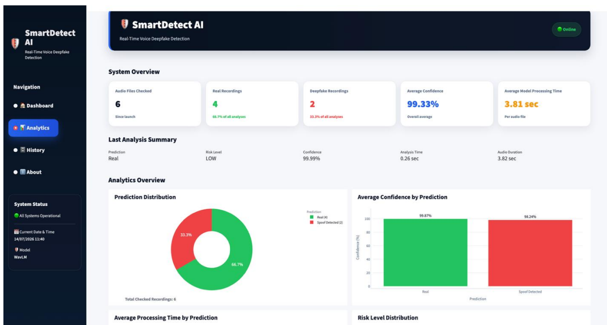
Figure 2. Analytics Page
