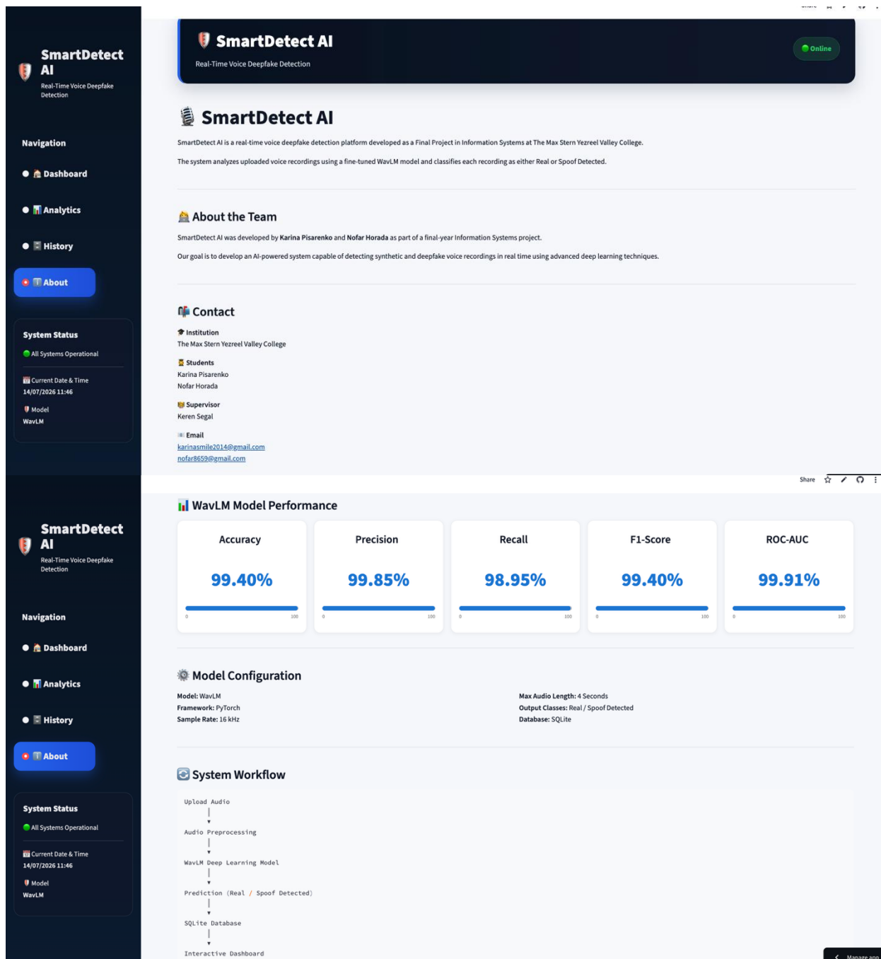
Figure 4. About page
